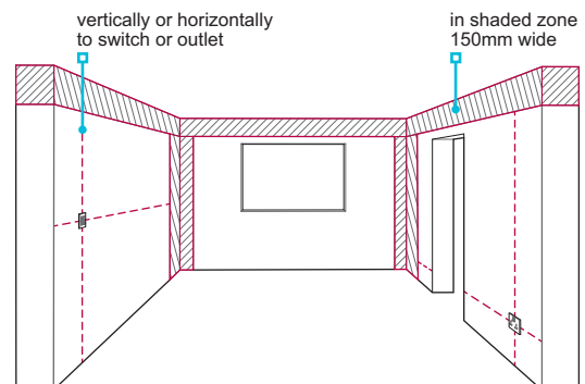
Figure 10: Safe location of cables
