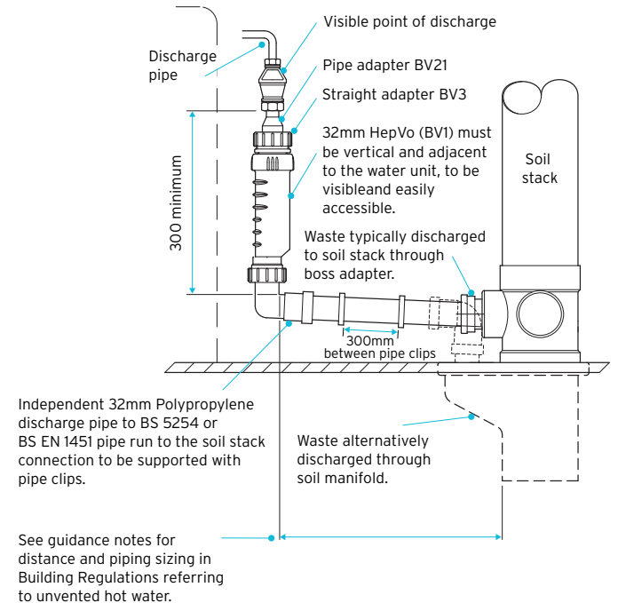
Figure 18: Unvented discharge – soil stack
