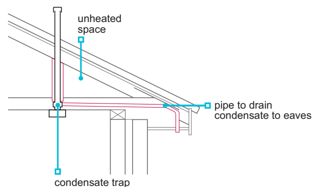
Figure 4: Ventilation control condensation - condense trap
