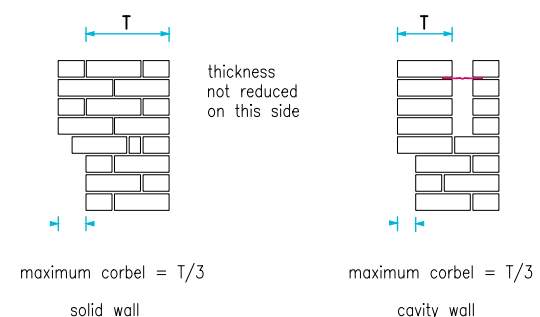
Figure 18: Corbelling
