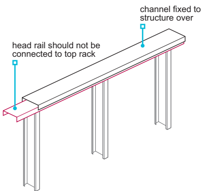
Figure 22: Deflection head
