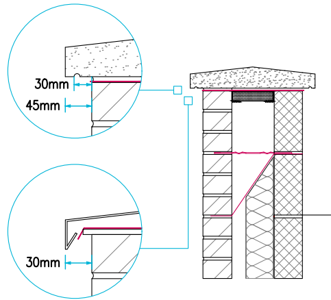
Figure 36: Copings/cappings to parapet walls
