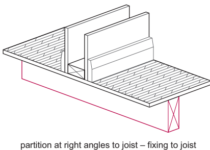
Figure 19: Partition fixing to joist
